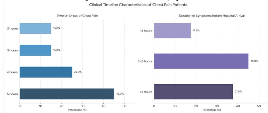
Fig 2: Time and duration of symptoms
