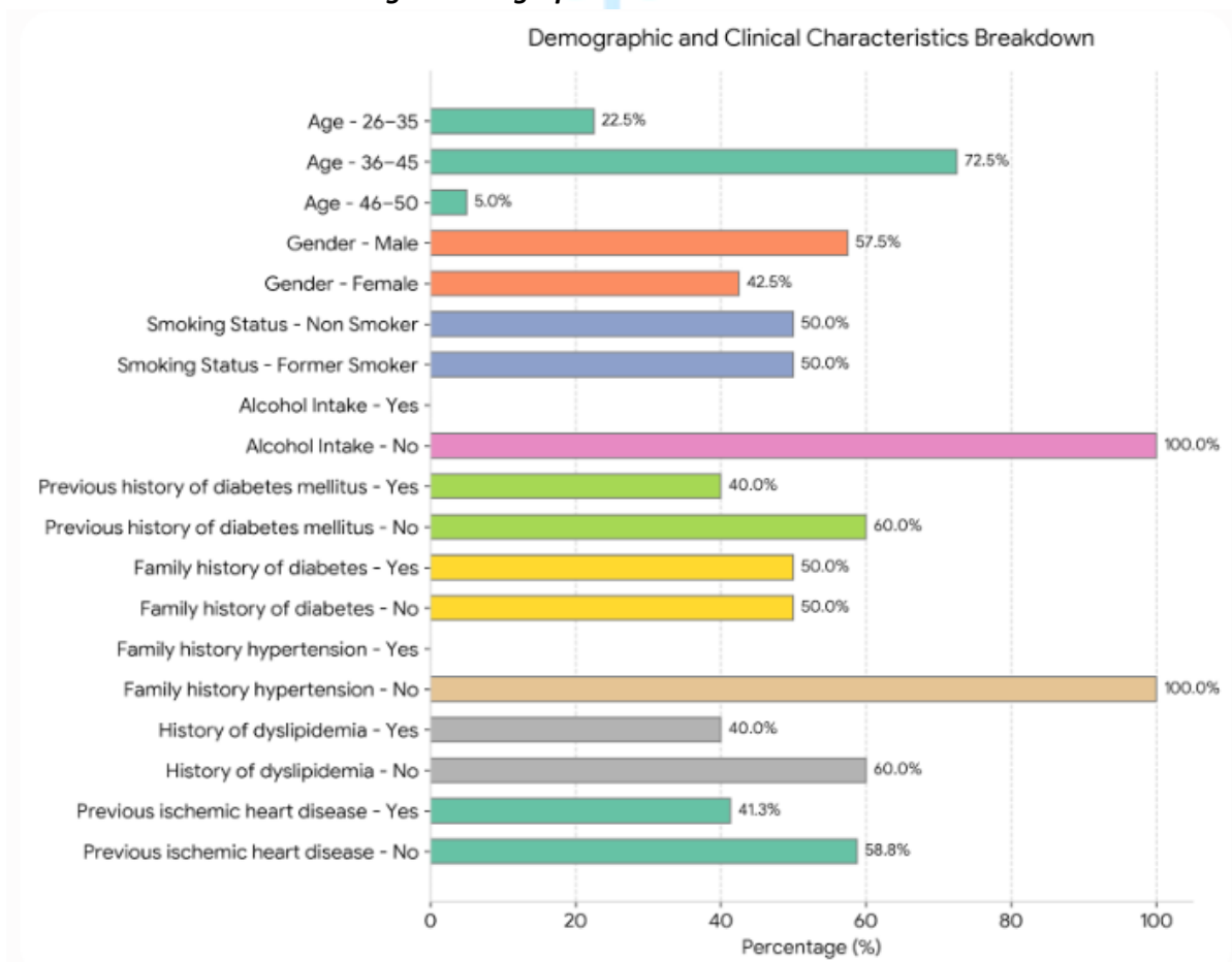
Fig 1: Demographic and disease histories
