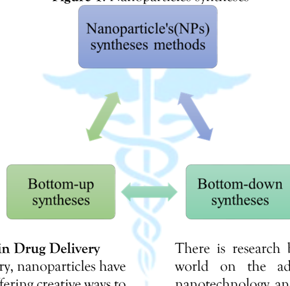
Figure 1: Nanoparticles syntheses
